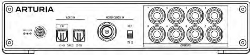
The AudioFuse X8 OUT rear panel
