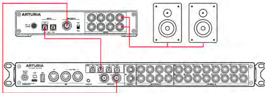
Hooking up the AudioFuse X8 OUT to your system
