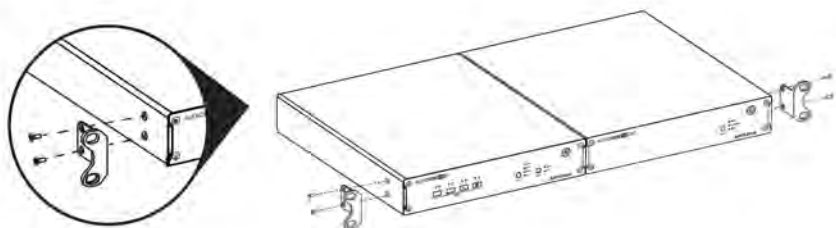
AudioFuse X8 IN configured for rackmounting
